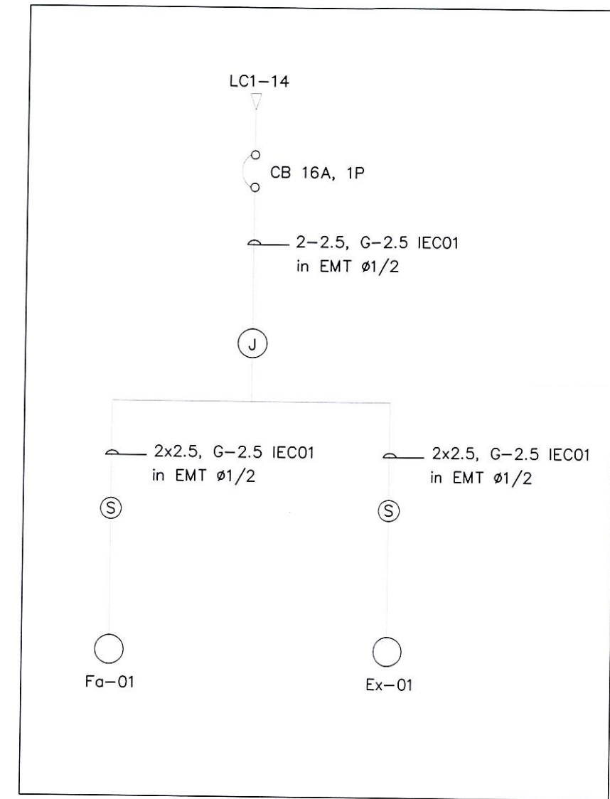
Single line diagram for FA-01 & Ex-01
